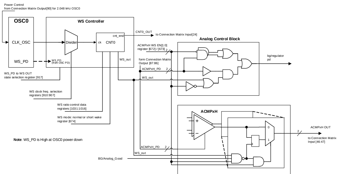
Figure 93: Wake/Sleep Controller
