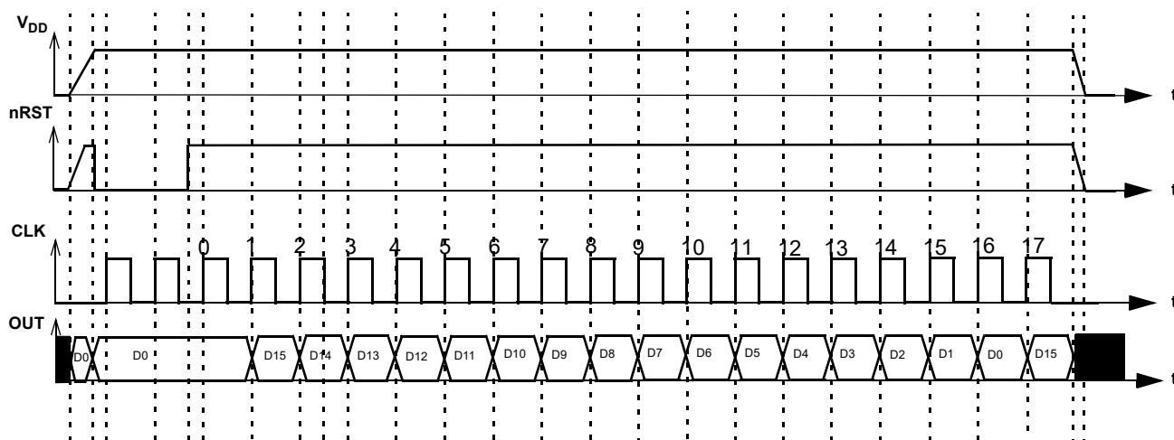
Figure 53: PGen Timing Diagram
