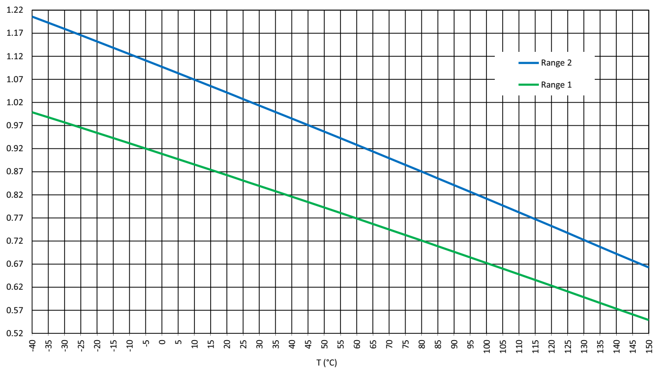
Figure 158: TS Output vs. Temperature, V_{DD} = 2.3\text{ V to }5.5\text{ V}
