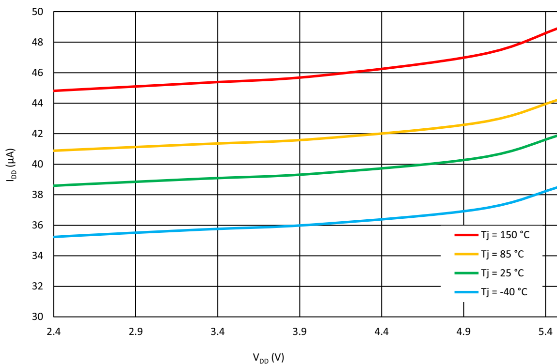
Figure 116: ACMPxH Current Consumption vs. V_{DD} at V_{ref} = 1024 mV
